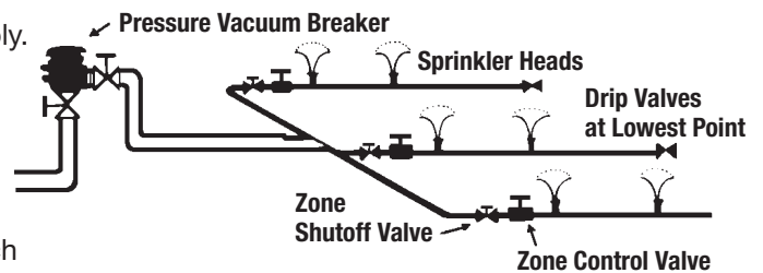
Multizone System
